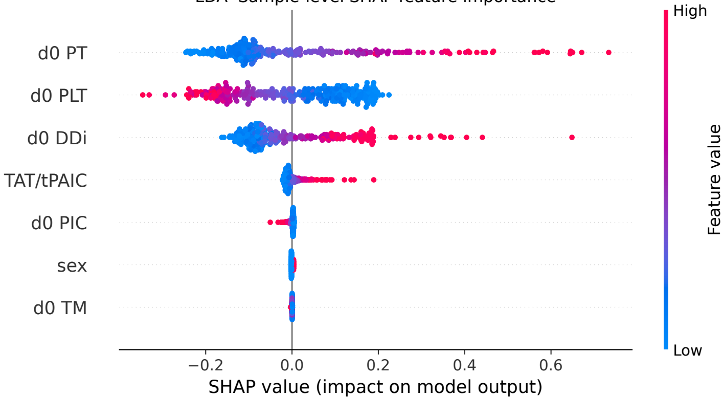
LDA Sample-level SHAP feature importance
